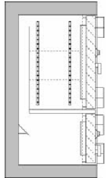
INTERIOR SIDE VIEW OF SAFE
